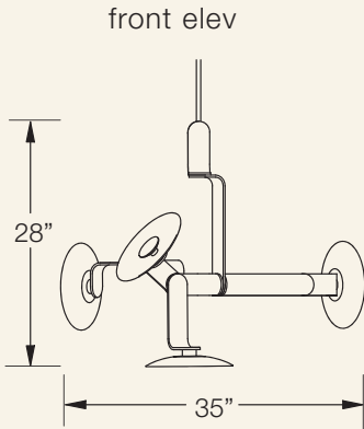
elbo-5.2 chandelier
