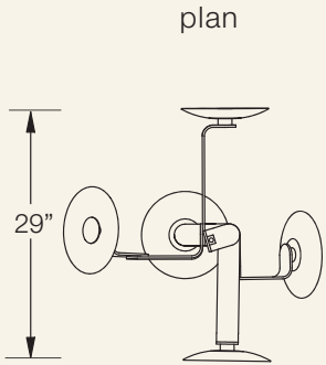
elbo-5.2 chandelier
